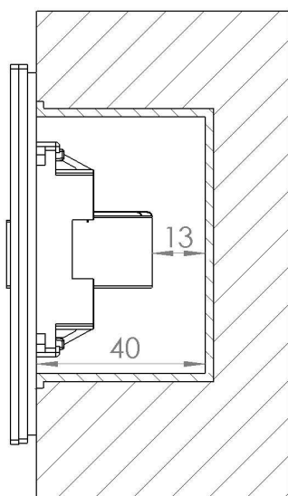
Height dimensions (size in mm)
